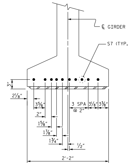
DETAIL "C" (FOR 63" & 72" MODIFIED BULB TEES)
