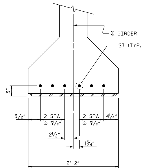
DETAIL "A" (FOR AASHTO TYPE IV GIRDERS)
